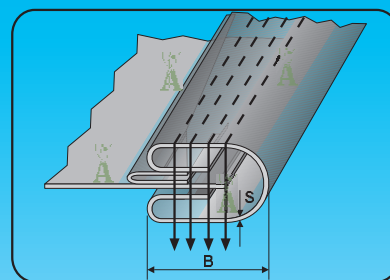
RIGHT ANGLE DOUBLE BINDER WITH PIPING
